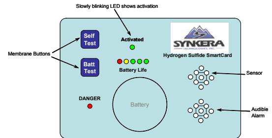
Figure 2. Proposed Alert Card Design. A very small, lightweight instrument, which takes advantage of the features of Synkera's unique electrochemical sensors.
