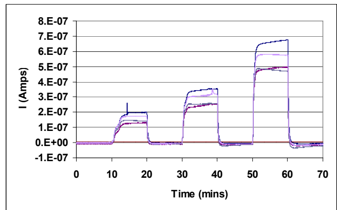
Figure 1: Sensor response to 5, 10 and 20 ppm H 2 S in a dry gas stream.
