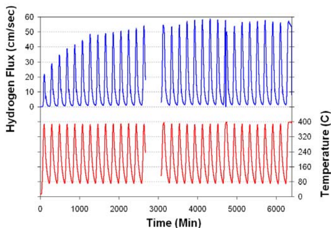
Temperature cycling performance of Synkera membrane (100% H 2 , 60 psi).
