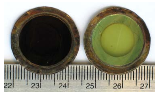
Prototypes of methanol reformer with metallic rim to facilitate sealing and integration.
