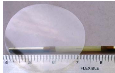
Planar (47 mm) and tubular (1/4") catalytic support substrates (thickness 0.1 mm).
