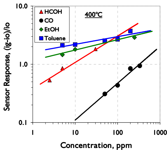
Sensitivity of SnO 2 microsensors to HCHO, CO, Toluene and EtOH at 400°C.
