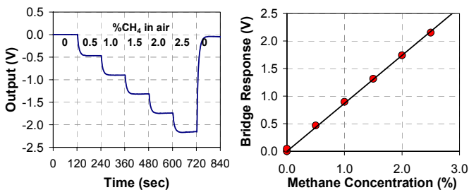
Output of the bridge circuit for varied CH 4 levels (left) and a linear calibration plot (right).
