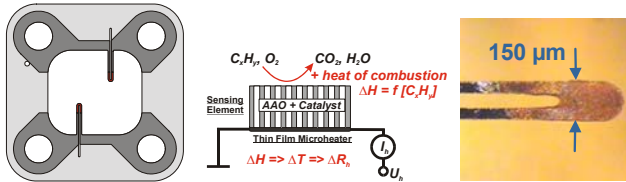
Representative sensor design, outline of the cross-section and the top view of the sensing element.
